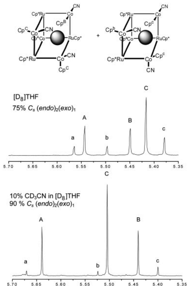
Figure 1. Schematic of the two detected isomers of \text{CsC}_4\text{Co}_4\text{Ru}_3 (top), ^1\text{H} NMR spectra of \text{CsC}_4\text{Co}_4\text{Ru}_3 in various solvents (bottom).
