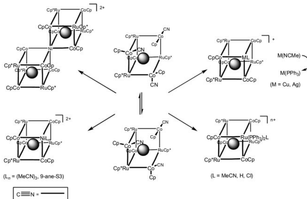
Scheme 1. Box-completion reactions of \text{CsC}_4\text{Co}_4\text{Ru}_3 described in this report.
