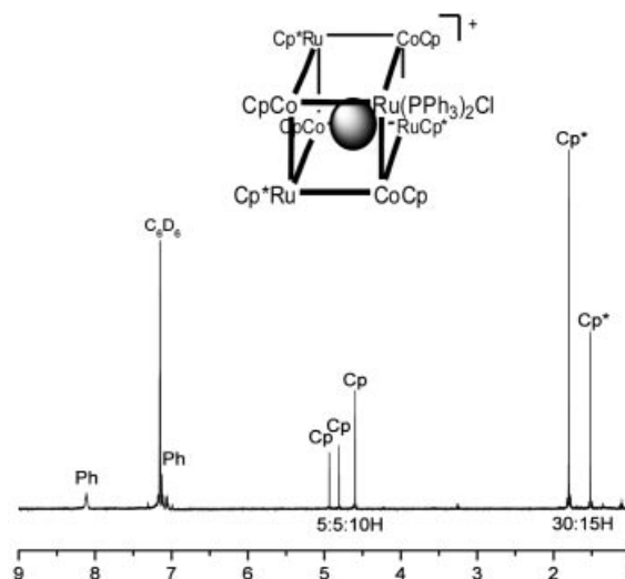
Figure 3. ^1\text{H} NMR spectrum of \{\text{Cs}[\text{CpCo}(\text{CN})_3]_4[\text{Cp}^*\text{Ru}]_3[\text{Ru}(\text{PPh}_3)_2\text{Cl}]\text{Cl} in \text{C}_6\text{D}_6 solution.
