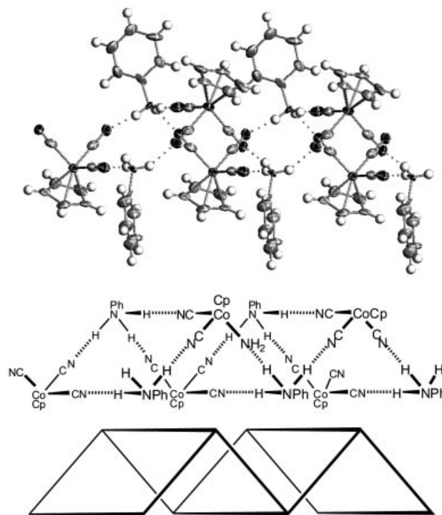
Figure 2. Structure of the hydrogen-bonded polymer \text{PhNH}_3\text{CpCo}(\text{CN})_3 (top). Schematic illustrating the bonding in the tape polymer (bottom).
