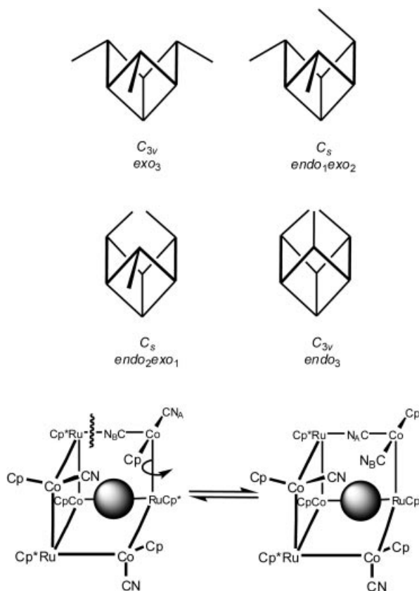
Scheme 2. Schematic depiction of isomers for the \text{M}_7 defect cages (top), and pathway that interconverts the two C_s isomers (bottom).
